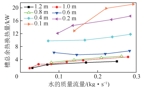
图6 模拟槽总余热换热量随水流量的变化 Fig.6 Variation of the total heat rate recovered with the water flow rate
