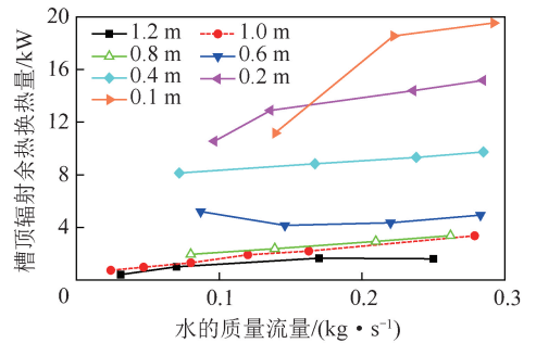
图5 模拟槽顶面辐射余热换热量随水流量的变化 Fig.5 Variation of the radiant heat rate recovered from the top of wall with the water flow rate
